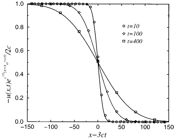
FIG. 1. f(y,t) = -u(x,t)\exp[\sqrt{c}(x-x_0-ct)]/2c vs y = x - 3ct for t = 10 (circle), 100 (diamond), and 400 (square), starting from the square-well initial condition u(x,0) = -V\theta(a - |x|) , with V = a = 1 . The solid line is the analytic approximation (5).
