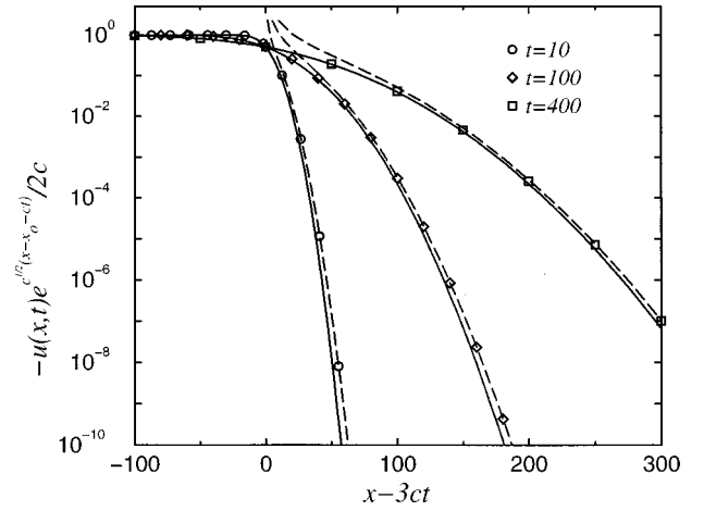
FIG. 2. Same data as in Fig. 1, in semilog scale, plotted together with the two overlapping approximations (5) (solid line) and (10) (dotted line).
